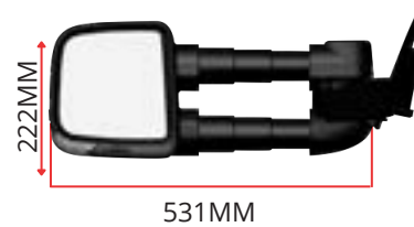
Fully Extended Towing Position
